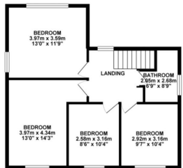
1ST FLOOR 57.78 sq. m. ( 621.95 sq. ft. )
