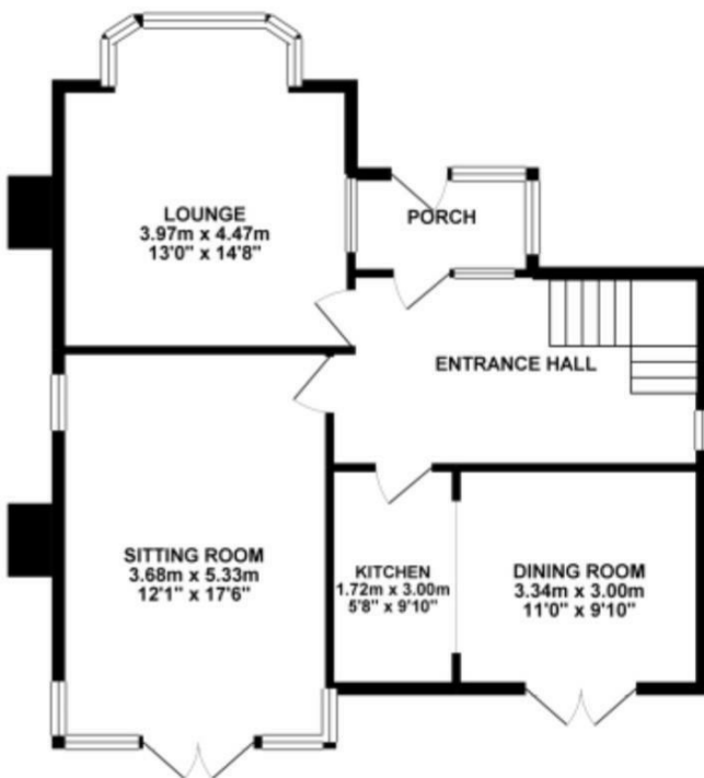
GROUND FLOOR 67.53 sq. m. ( 726.88 sq. ft. )
